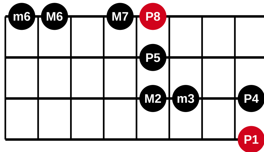
4 strings - 8 frets - fingering 32 of 56
