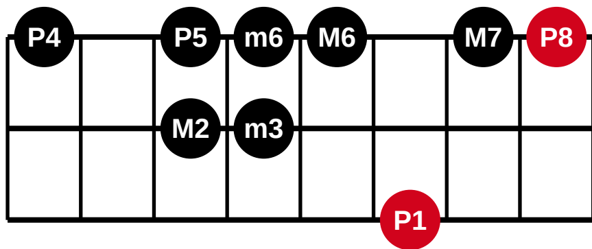
3 strings - 8 frets - fingering 20 of 28
