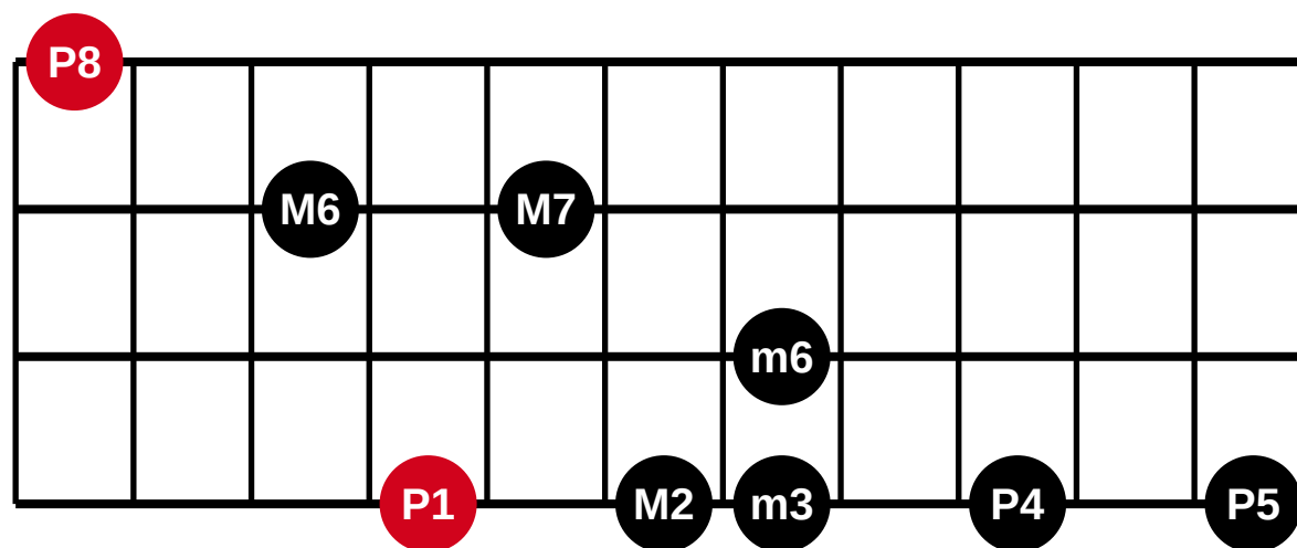
4 strings - 11 frets - fingering 49 of 56
