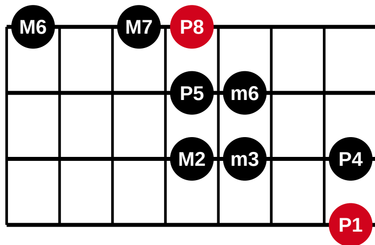
4 strings - 7 frets - fingering 17 of 56
