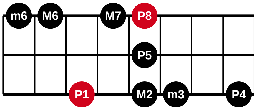
3 strings - 8 frets - fingering 18 of 28
