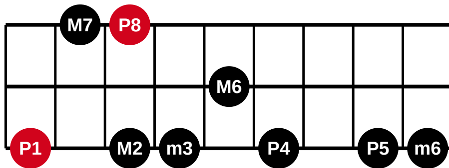
3 strings - 9 frets - fingering 22 of 28
