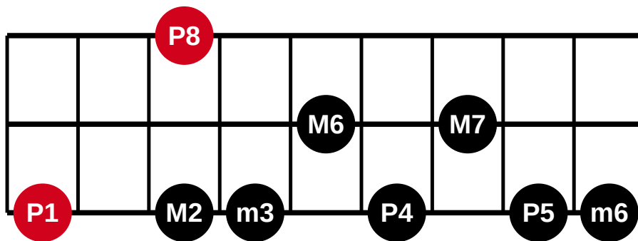
3 strings - 9 frets - fingering 23 of 28
