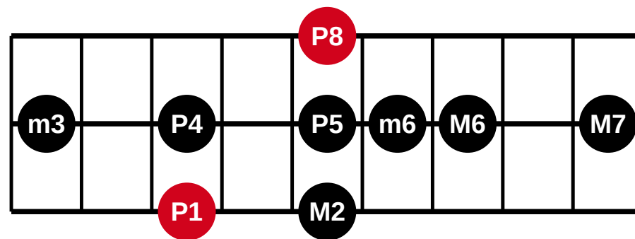
3 strings - 9 frets - fingering 25 of 28
