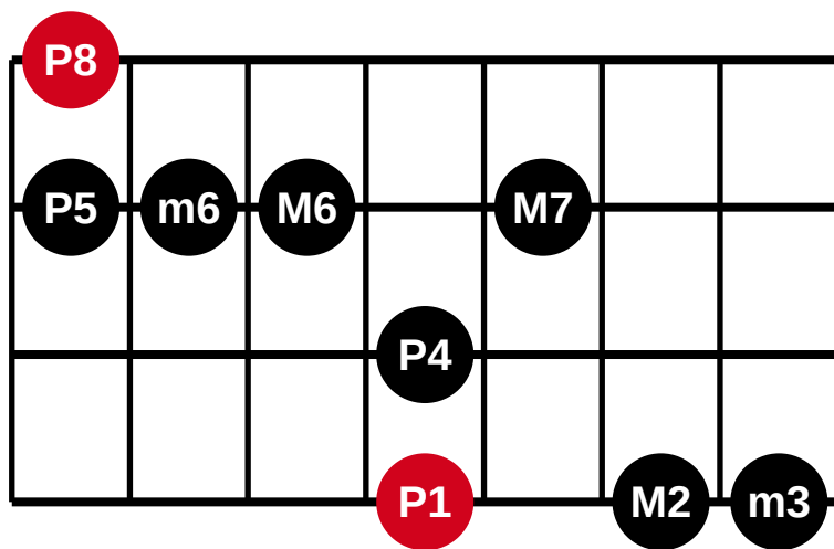
4 strings - 7 frets - fingering 9 of 56
