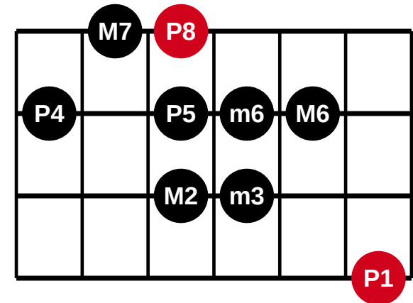
4 strings - 6 frets - fingering 6 of 56
