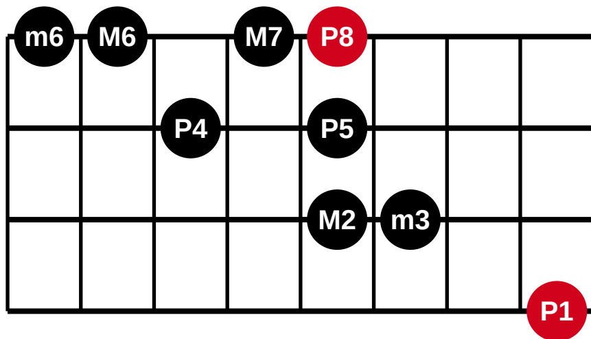
4 strings - 8 frets - fingering 31 of 56
