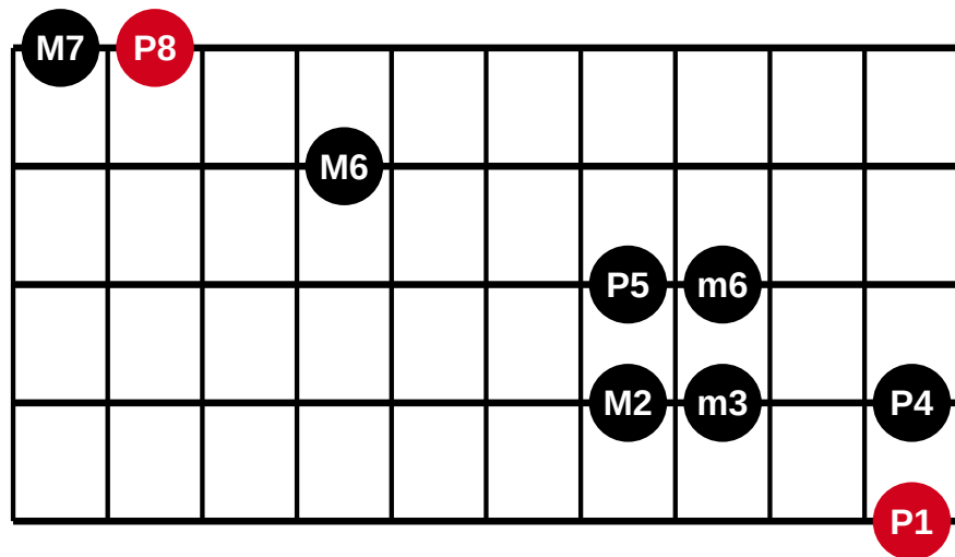
5 strings - 10 frets - fingering 19 of 70
